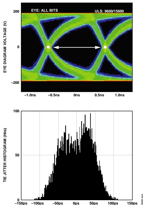
Figure 51. Data Eye for LVDS Outputs in ANSI-644 Mode with Trace Lengths Greater than 24 Inches on Standard FR-4, External 100 Ω Far Termination Only
