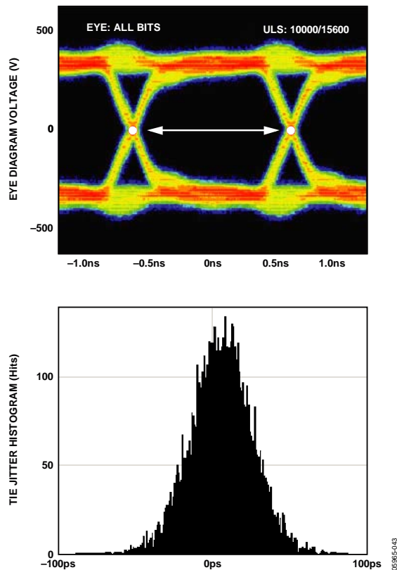
Figure 50. Data Eye for LVDS Outputs in ANSI-644 Mode with Trace Lengths Less than 24 Inches on Standard FR-4, External 100 Ω Far Termination Only
