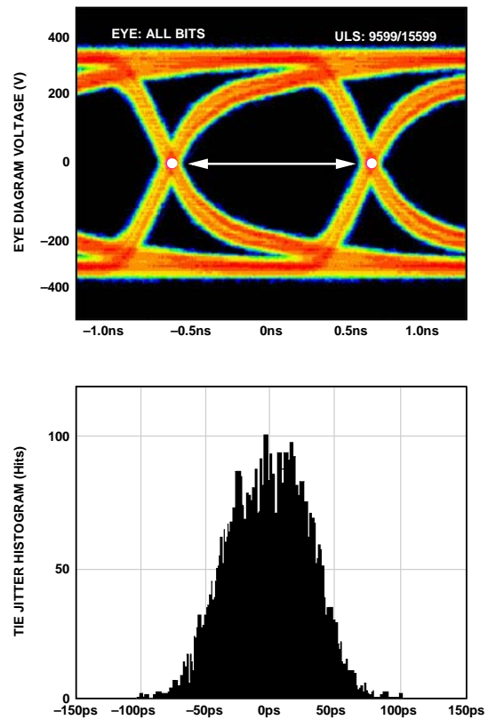
Figure 52. Data Eye for LVDS Outputs in ANSI-644 Mode with 100 Ω Internal Termination on and Trace Lengths Greater than 24 Inches on Standard FR-4, External 100 Ω Far Termination Only
