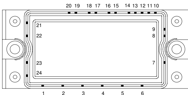
APTGS25X120RTP2: Without Brake (Pin 7 & 14 not connected)
