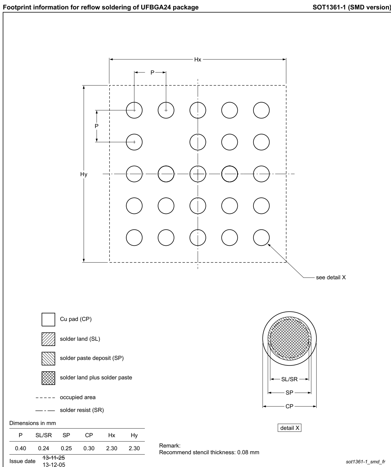
Fig 50. PCB footprint for SOT1361-1 (UFBGA24, Solder Mask Defined version), ER option; reflow soldering
