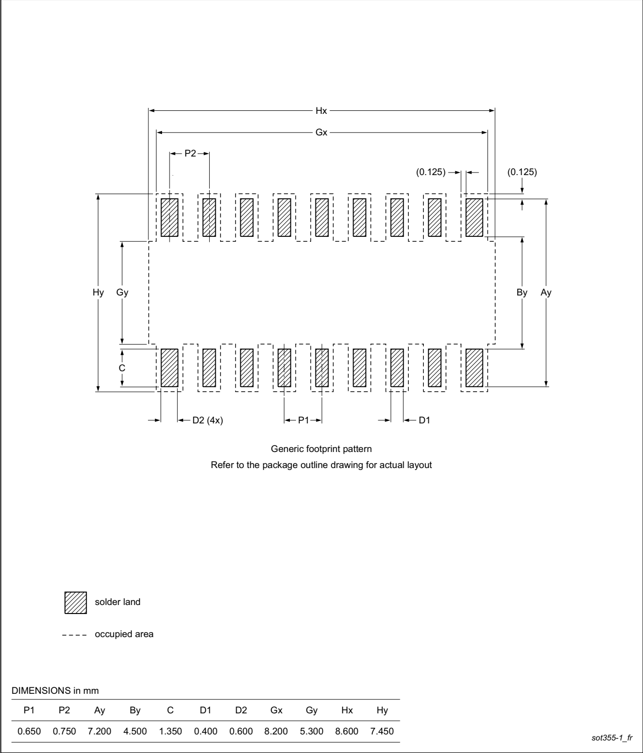
Fig 45. PCB footprint for SOT355-1 (TSSOP24); reflow soldering
