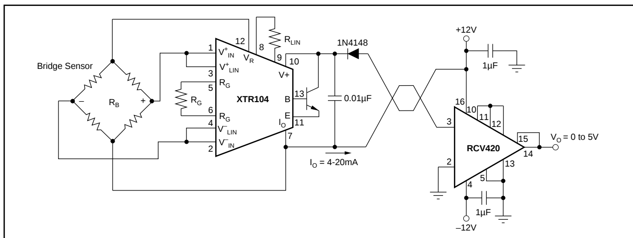
FIGURE 9. \pm 12\text{V} -Powered Transmitter/Receiver Loop.
