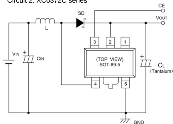
Circuit 2: XC6372C series
