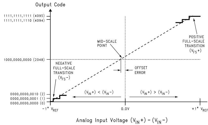
Figure 2. Transfer Characteristic
