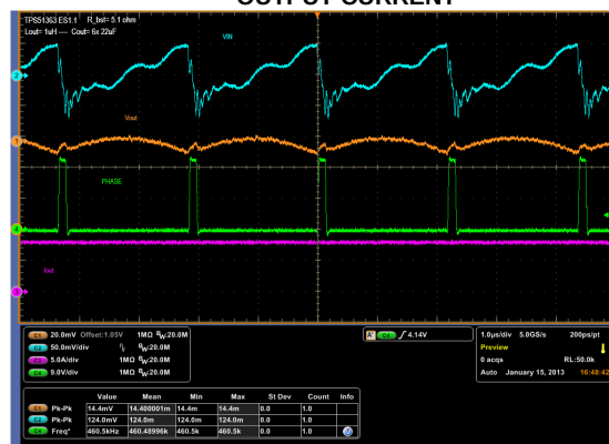
Figure 18. f = 400\text{kHz} , V_{\text{IN}} = 20\text{V} , I_{\text{OUT}} = 8\text{A}
