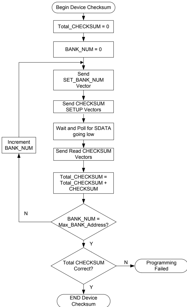
Figure 3-14. Verify Checksum Procedure
