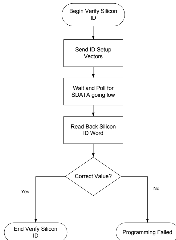
Figure 3-7. Verify Silicon ID Procedure
