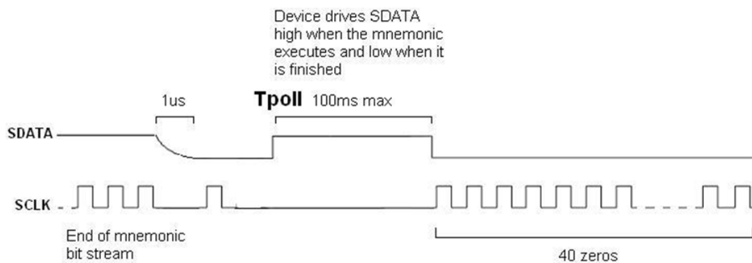
Figure 3-3. “Wait and Poll” Timing Diagram
