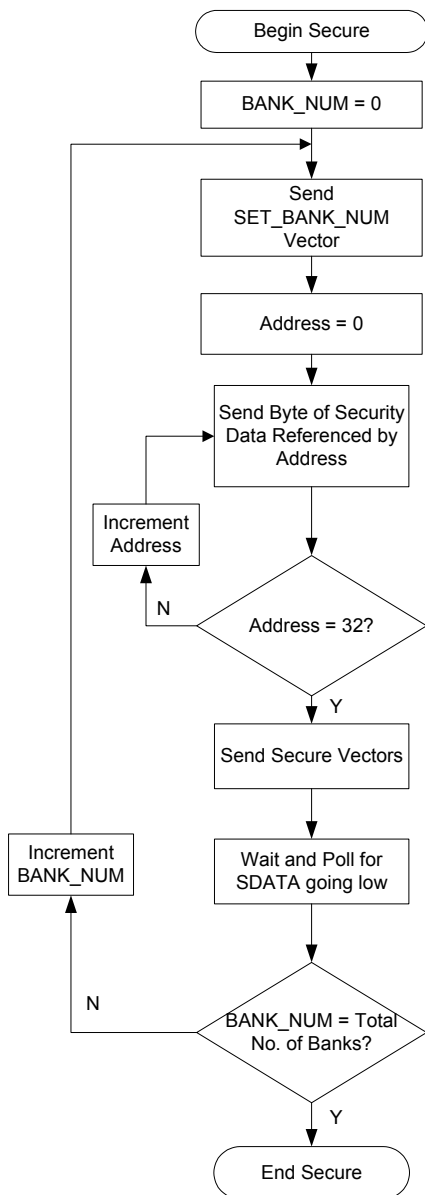
Figure 3-13. Secure Procedure
