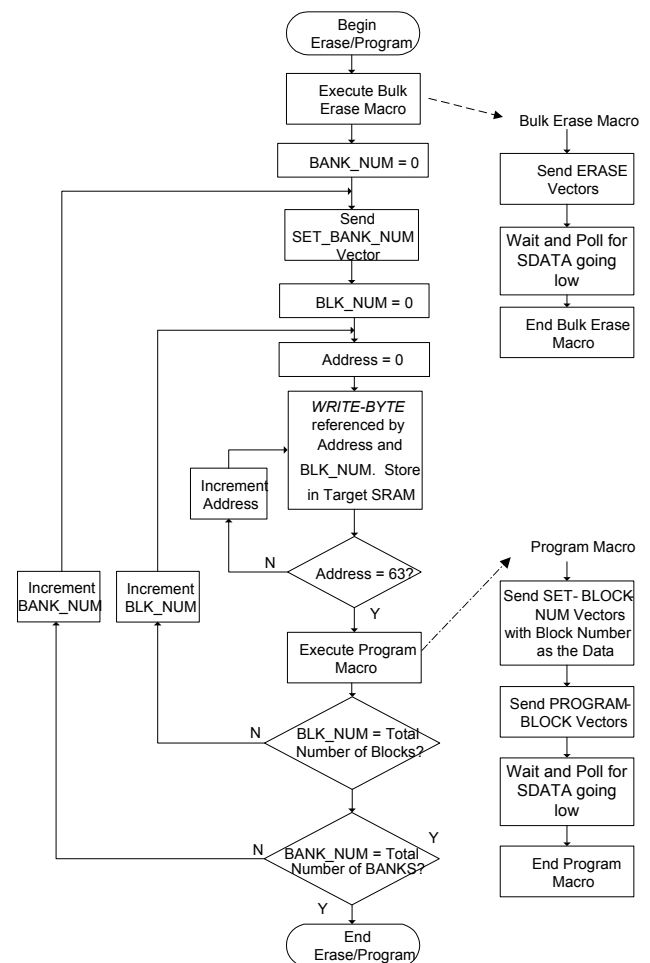
Figure 3-9. Program Procedure
