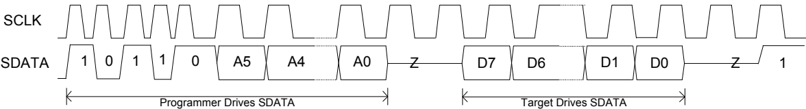
Figure 3-11. READ-BYTE From Target for Verify operation
