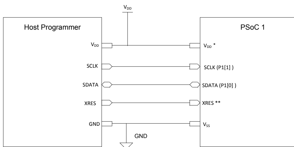
Figure 2-1. Host Programmer - PSoC 1 Interface
