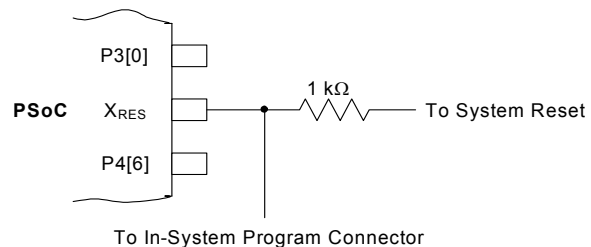
Figure 2-3. XRES Connection
