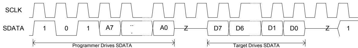
Figure 3-8. READ-BYTE (D7..D0) from Target PSoC 1 (At address A7..A0)
