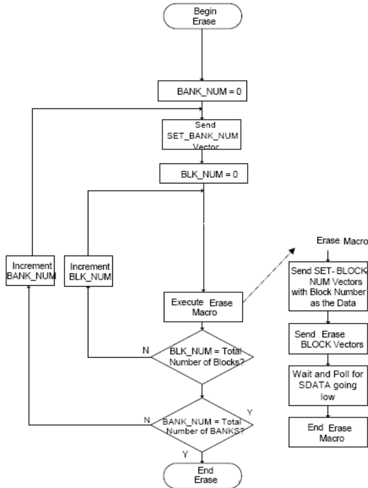
Figure 3-15. Erase Block Procedure
