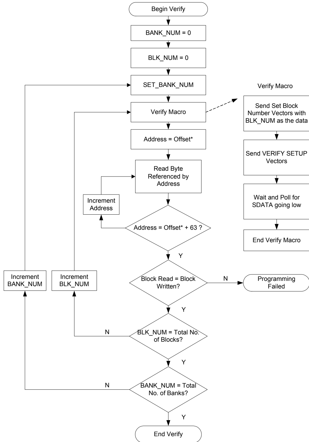
Figure 3-12. Verify Procedure (Offset = 0x80 in figure)
