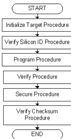
Figure 3-1. Target Programming Flow
