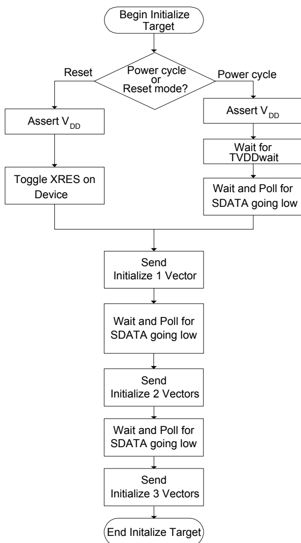
Figure 3-4. Initialize Target Procedure
