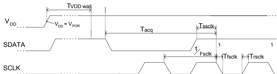
Figure 3-6. Using Power Cycling to Initialize
