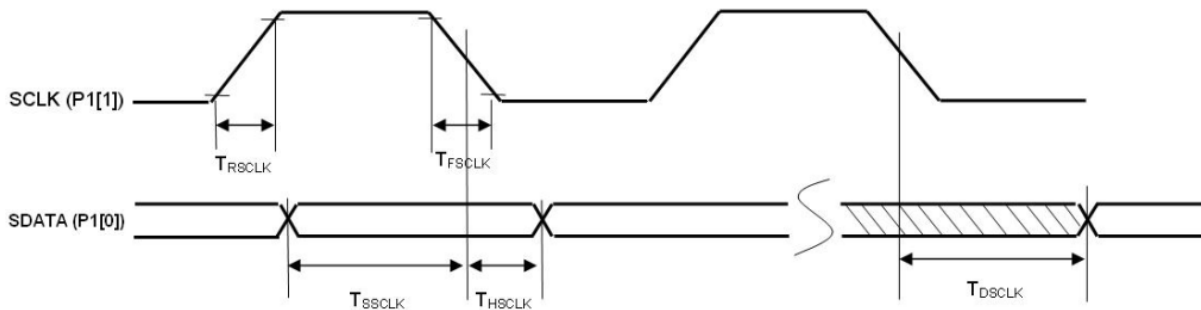
Figure 3-2. SCLK, SDATA Timing Diagrams
