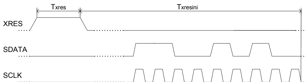
Figure 3-5. Using Reset to Initialize
