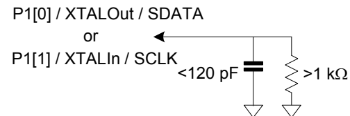
Figure 2-2. Maximum Load Data and SCLK Pins
