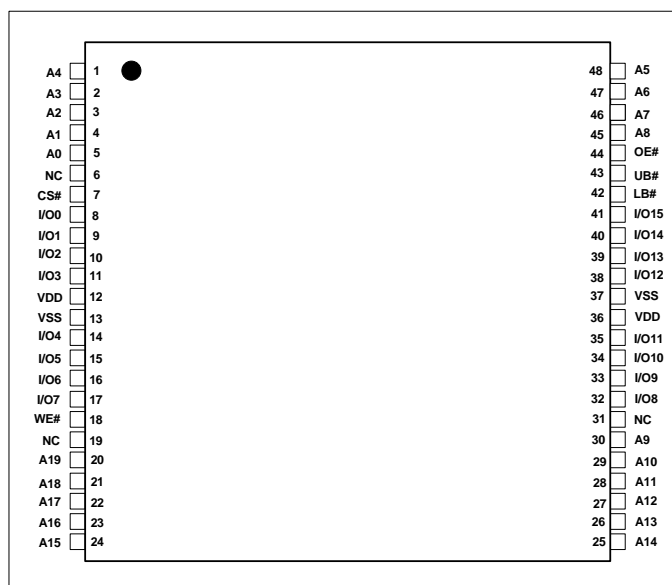
48-Pin TSOP ,TYPE I ( 12mm x 20mm )
