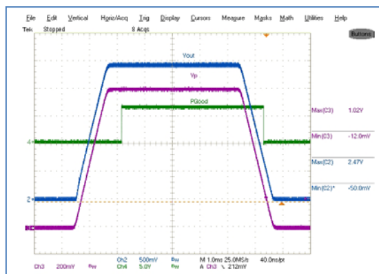
Figure 46: Voltage Tracking using Vp Pin, CH_2 -Vout, CH_3 -Vp, CH_4 -PGood
