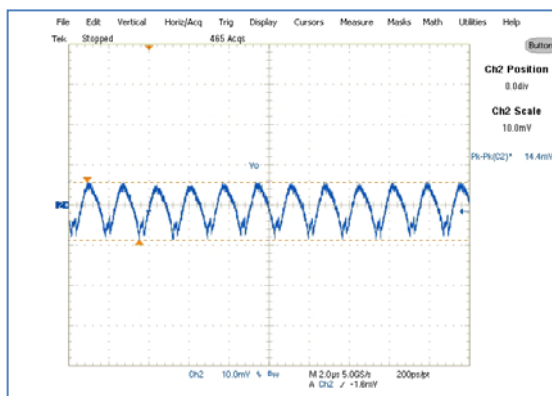
Figure 33: Output Voltage Ripple, 9A Load, Ch2:V out
