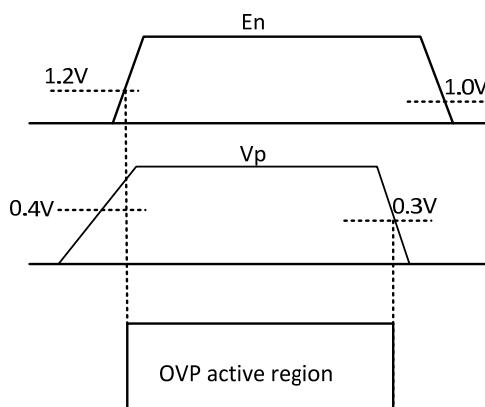
Figure 18b: Activation of OVP in tracking mode
