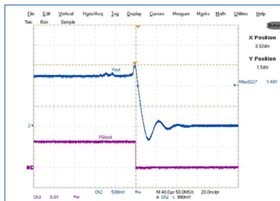
Figure 44: Over Voltage protection, CH_2 -Vout, CH_3 -PGood
