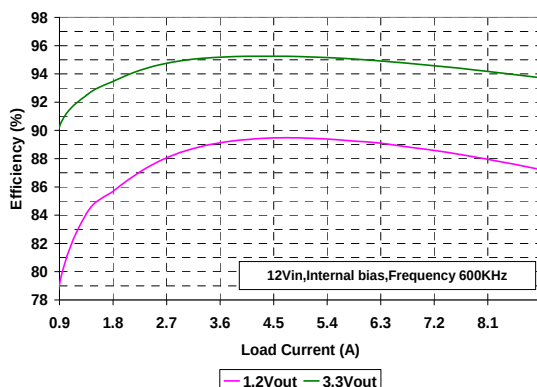
Figure 2: IR3899 Efficiency
