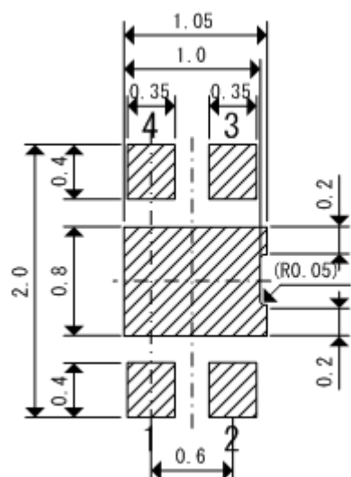
●USP-4D Reference Pattern Layout Dimension
