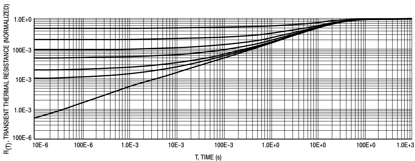
Figure 7. Thermal Response
