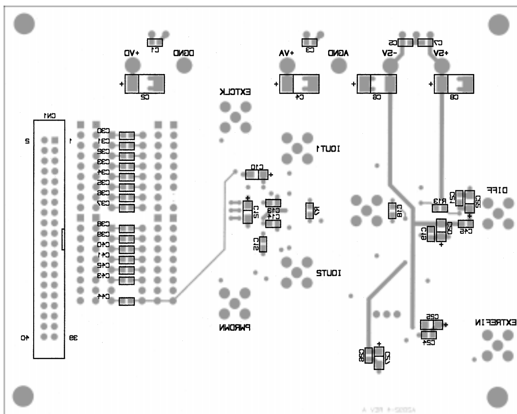
FIGURE 8. Bottom Layer with Silk-Screen (U-board).
