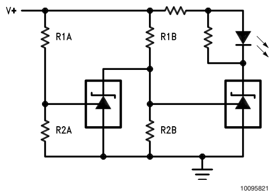
Voltage Monitor
