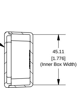
SECTION A-A End View of Assembly
