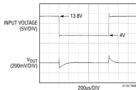
Fast (10µs) Cold Crank Line Transient, V_{IN} = 13.8V to 4V
