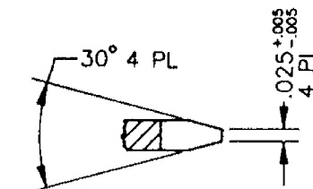
PARTIAL SECTION A-A
