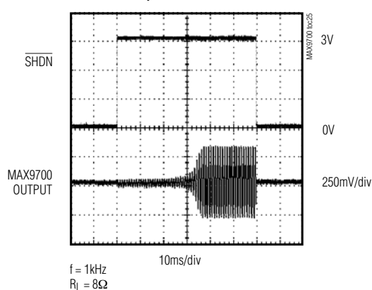
TURN-ON/TURN-OFF RESPONSE
