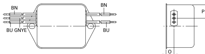
Connection style -08, 20 and 30A types
