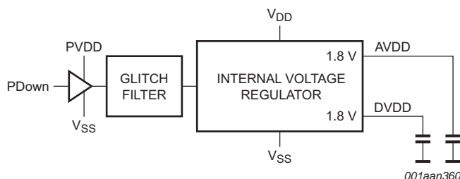
Fig 28. Internal PDown to voltage regulator logic
