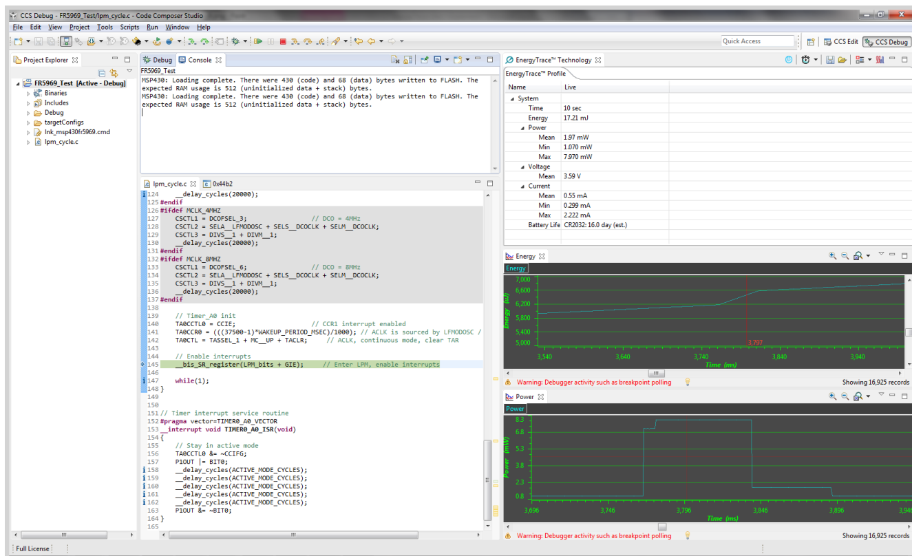
Figure 4-16. Debug Session With EnergyTrace Graphs
