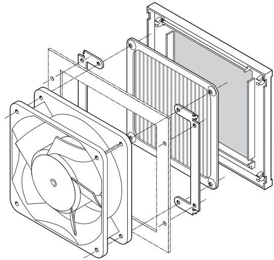
Bracket
