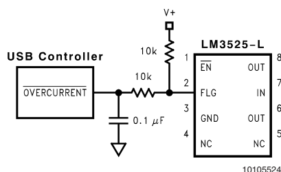
FIGURE 1. Transient Fitter
