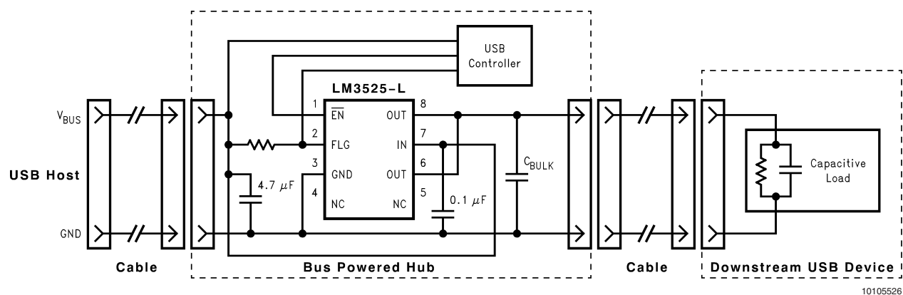
FIGURE 4. Soft-Start Application
