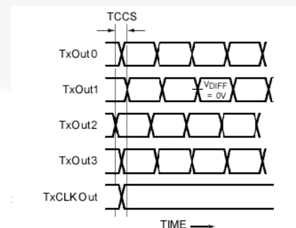
Figure 11. Transmitter Outputs Channel-to-Channel Skew
