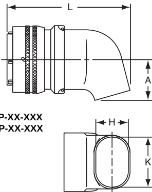
“SP” Potting Boot 75 degrees
