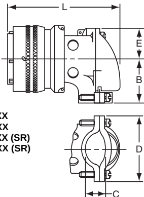
“SE” Open Wire Seal, “SE” (SR) Strain Relief
