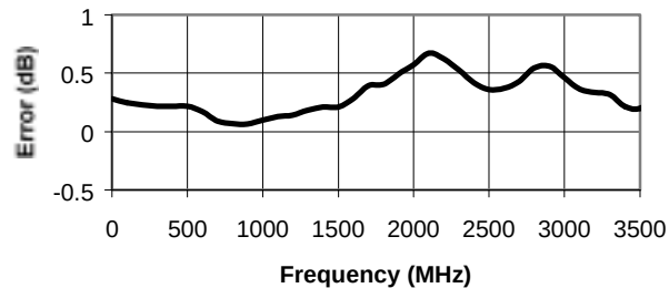
Attenuation Error 8 dB Bit
