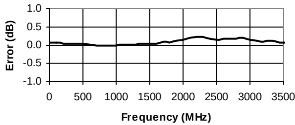
Attenuation Error 0.5 dB Bit
