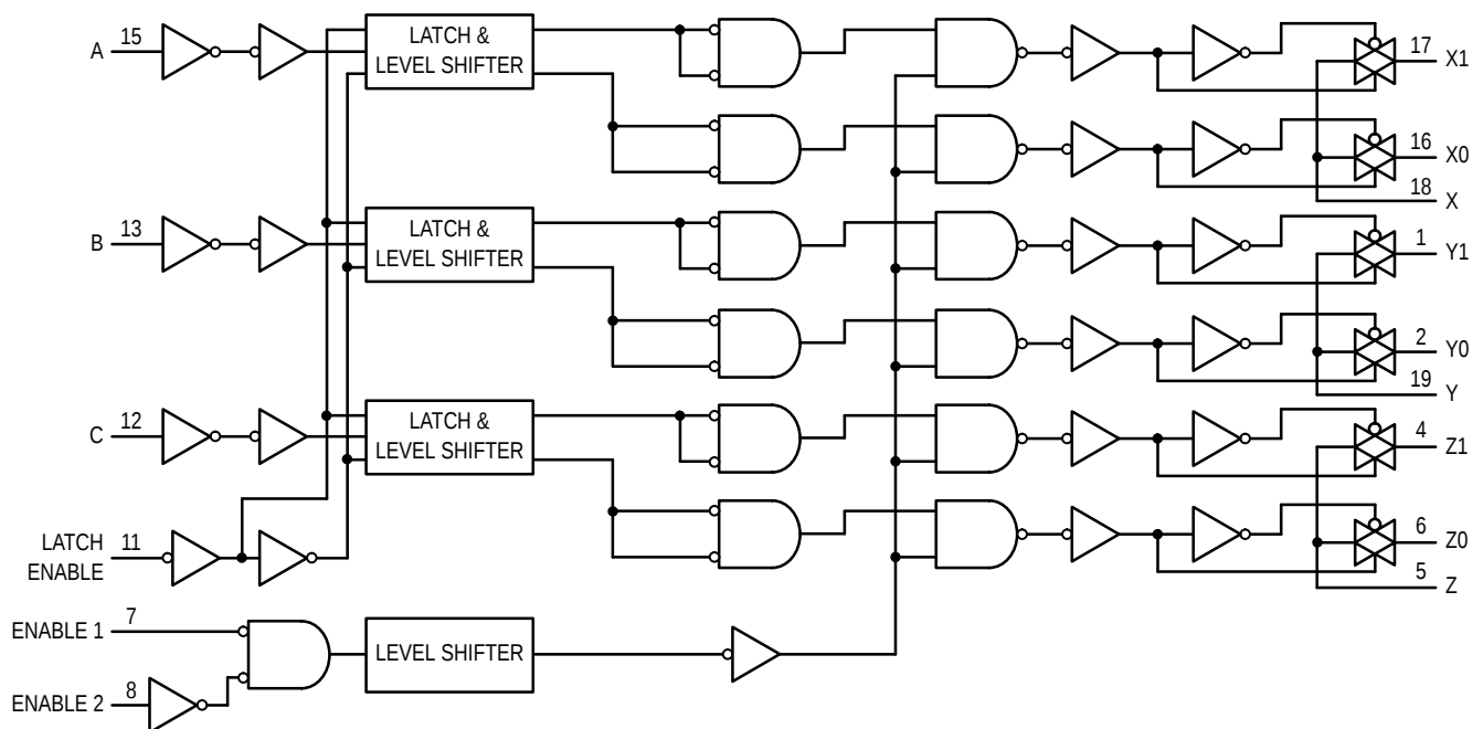
FUNCTION DIAGRAM HC4353
