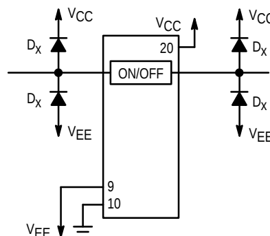
Figure 17. External Germanium or Schottky Clipping Diodes
