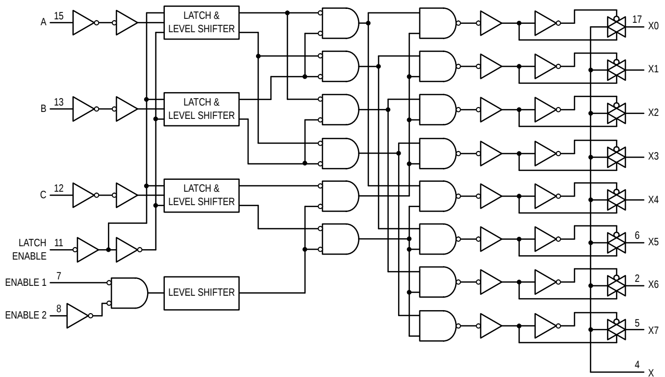
FUNCTION DIAGRAM HC4351
