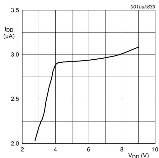
Fig 8. I_{DD} with respect to V_{DD}
