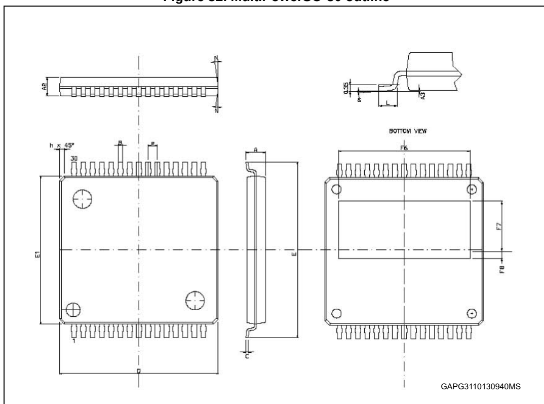
Figure 32. MultiPowerSO-30 outline
