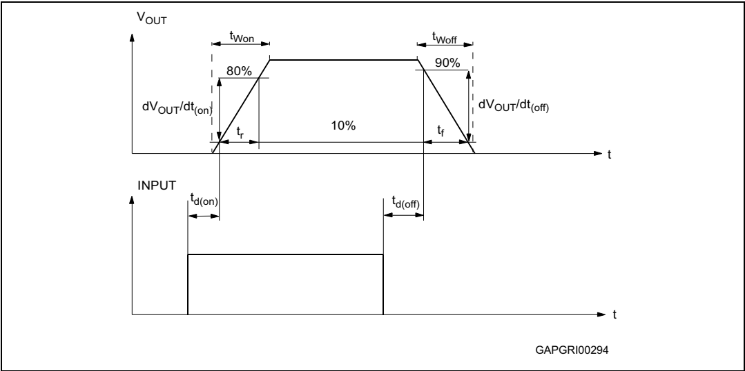
Figure 5. Switching characteristics
