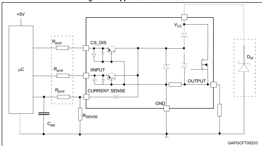
Figure 22. Application schematic
