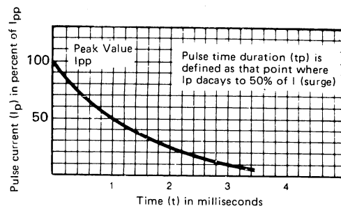
FIG. 2. Pulse wave form for exponential surge
