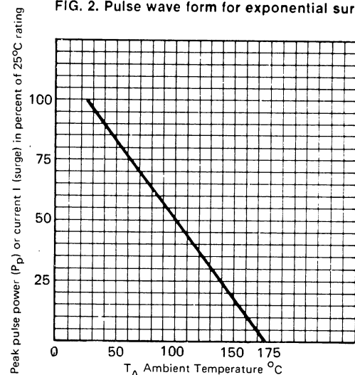
FIG. 3. Derating curve
