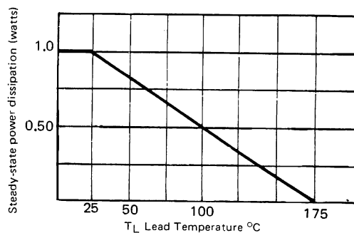
FIG. 4. Steady-state power derating curve
