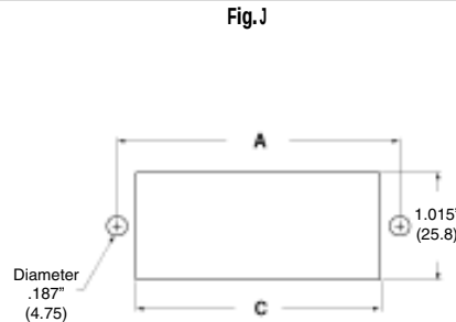
P Solder Hook (Standard)
