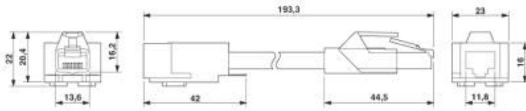
Dimensional drawing
