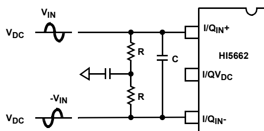
FIGURE 16. DC COUPLED DIFFERENTIAL INPUT
