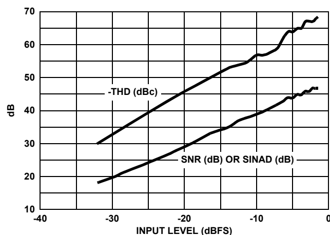
FIGURE 6. SINAD, SNR AND -THD vs INPUT AMPLITUDE
