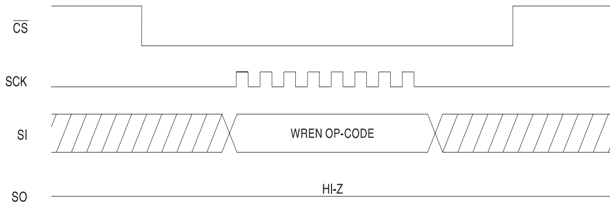
Figure 4. WREN Timing
