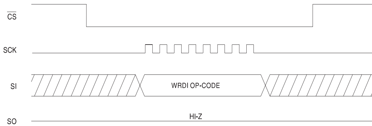
Figure 5. WRDI Timing
