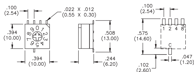
Mechanical outline
