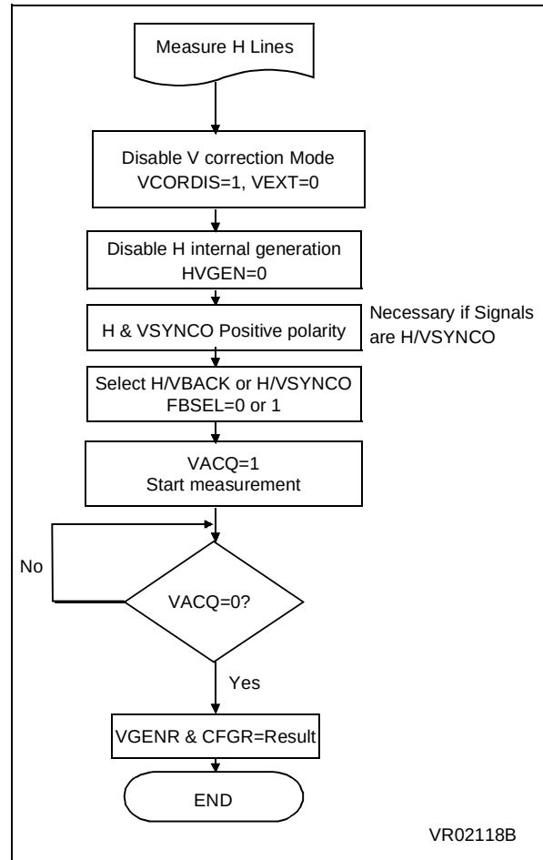
Figure 46. Vertical Output Measurement
