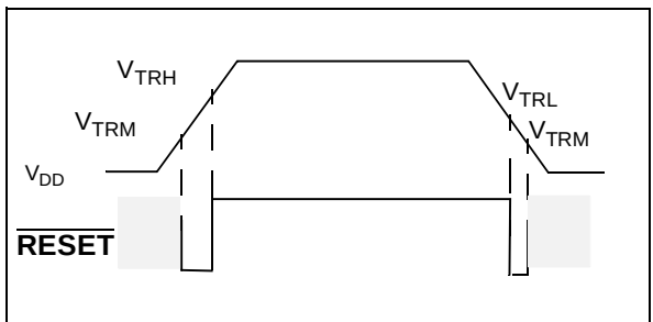
Figure 11. LVD Reset Signal Output
