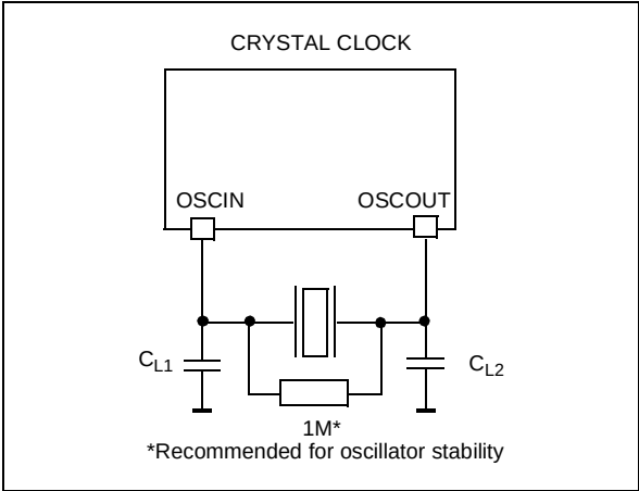
Figure 8. Crystal/Ceramic Resonator
