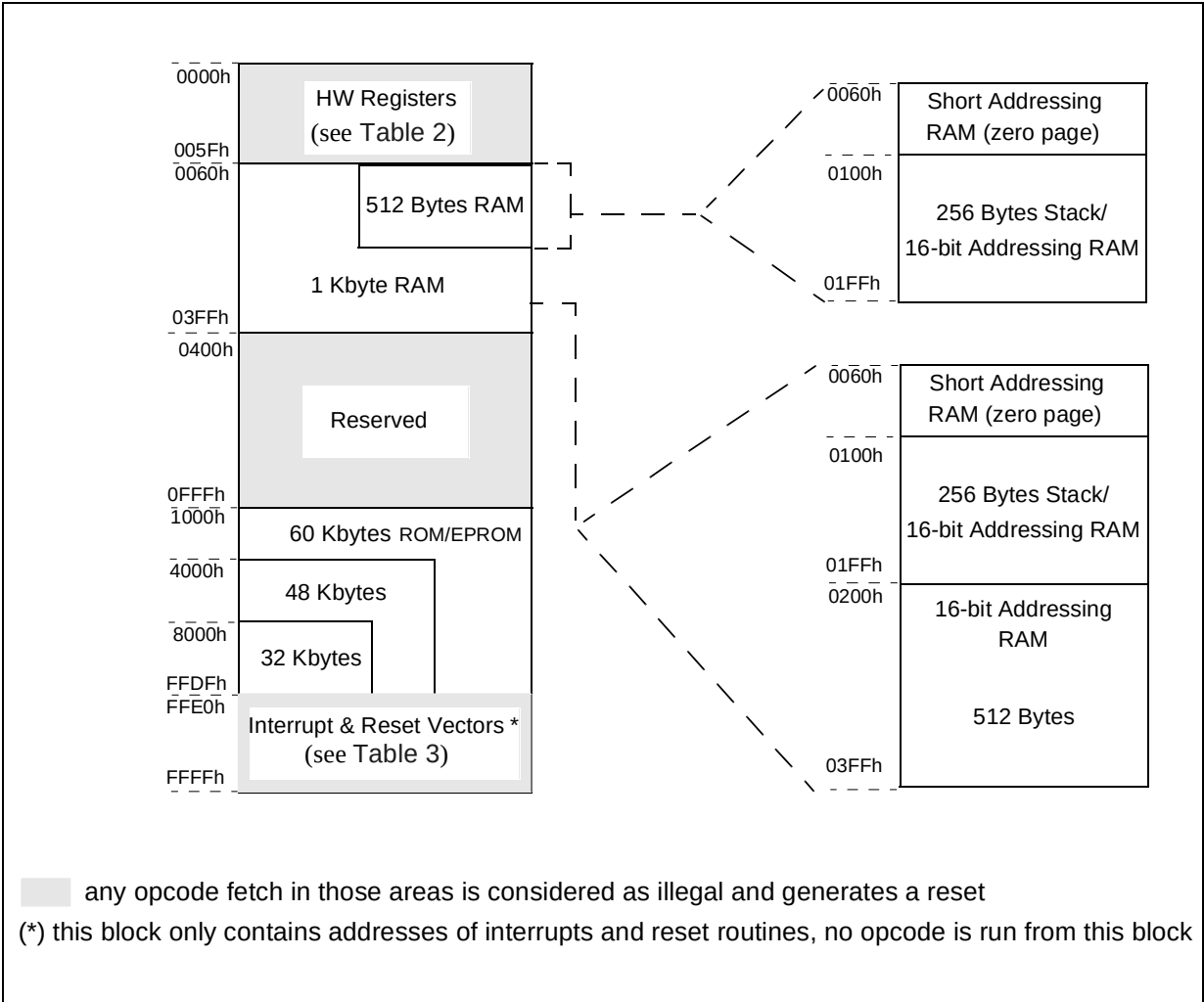
Figure 3. Memory Map
