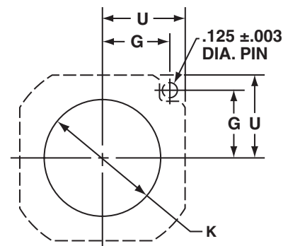
MOUNTING DIMENSIONS
