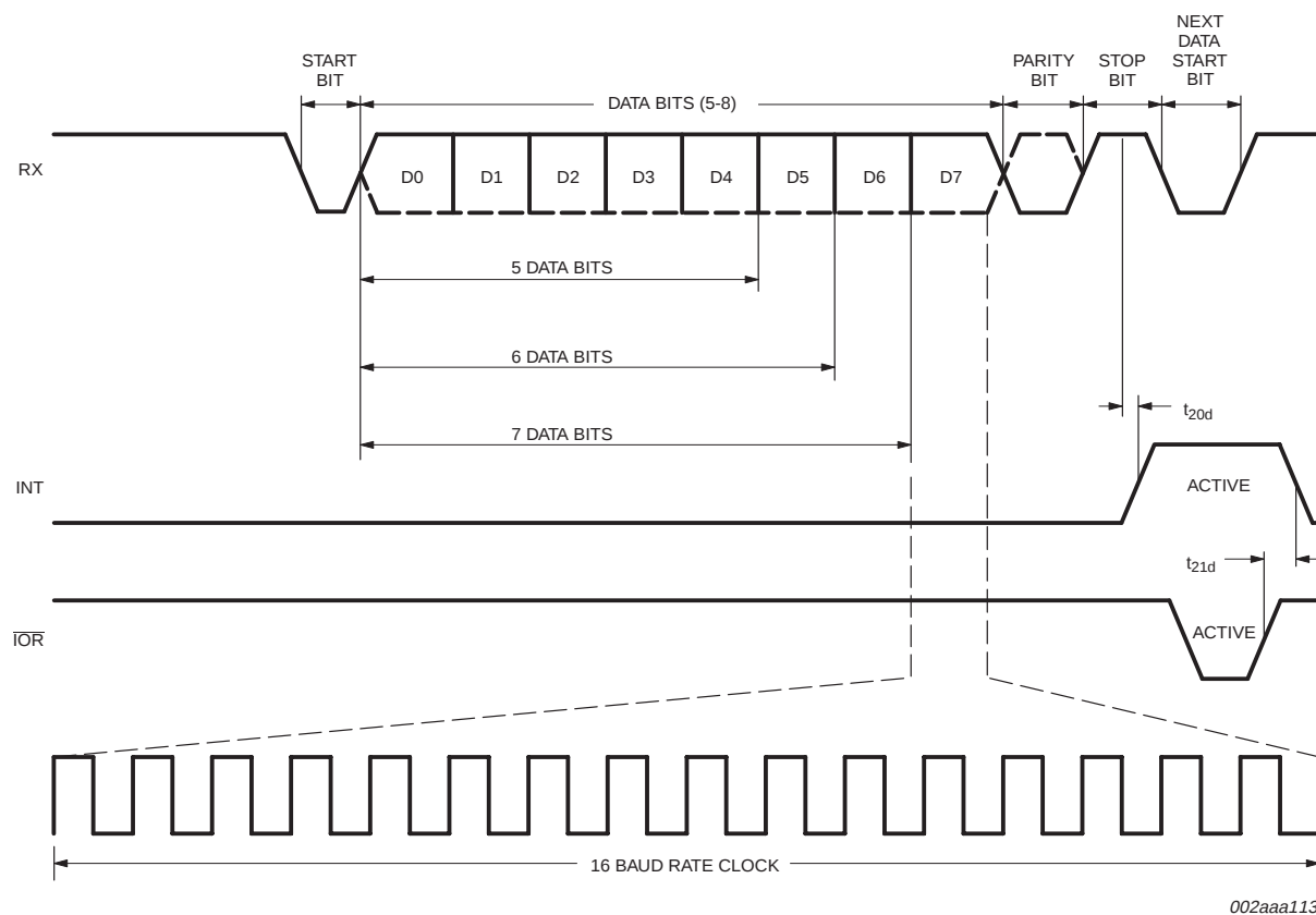
Fig 15. Receive timing.
