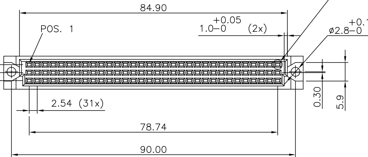
DETAIL B
