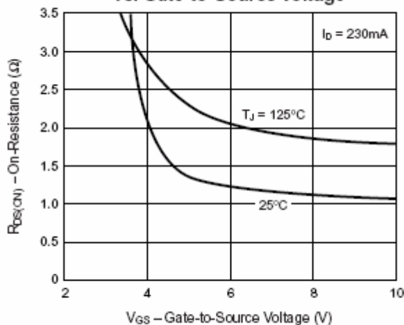
Fig. 1 – On-Resistance vs. Gate-to-Source Voltage
