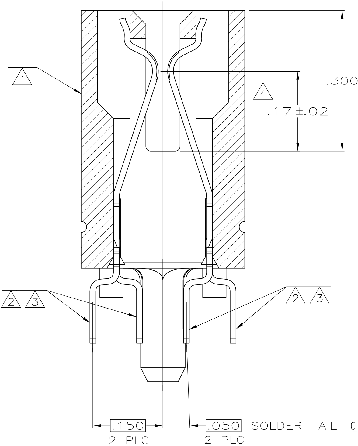
SECTION L-L SCALE 8:1
