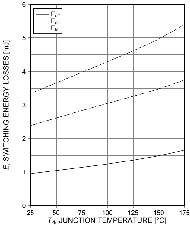
Figure 13. Typical switching energy losses as a function of junction temperature (inductive load, V_{CE}=400V , V_{GE}=0/15V , I_C=75A , R_{Gon}=18\Omega , R_{Goff}=5.6\Omega , dynamic test circuit in Figure E)
