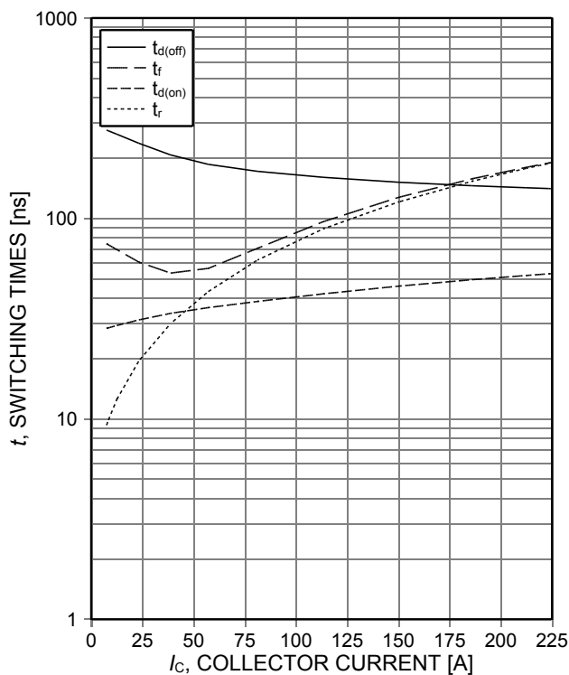
Figure 7. Typical switching times as a function of collector current (inductive load, T_{vj}=150^{\circ}C , V_{CE}=400V , V_{GE}=0/15V , R_{Gon}=18\Omega , R_{Goff}=5.6\Omega , dynamic test circuit in Figure E)
