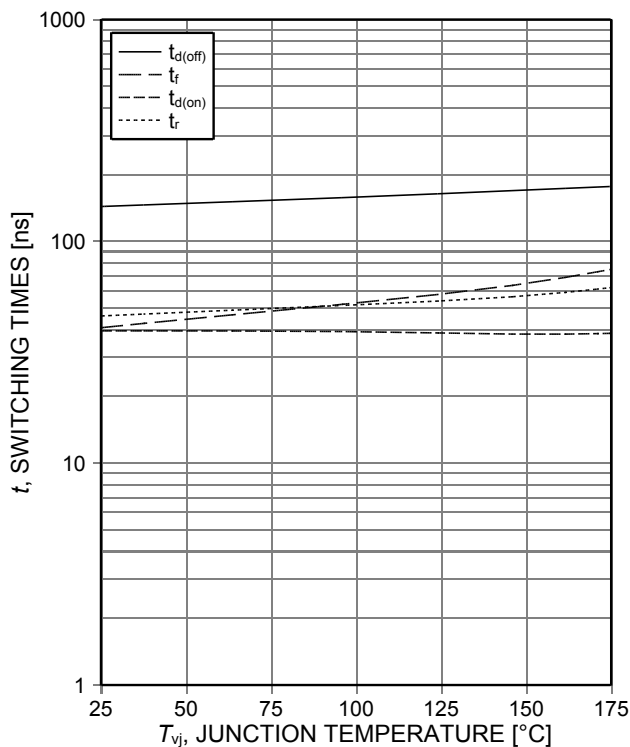
Figure 9. Typical switching times as a function of junction temperature (inductive load, V_{CE}=400V , V_{GE}=0/15V , I_C=75A , R_{Gon}=18\Omega , R_{Goff}=5.6\Omega , dynamic test circuit in Figure E)
