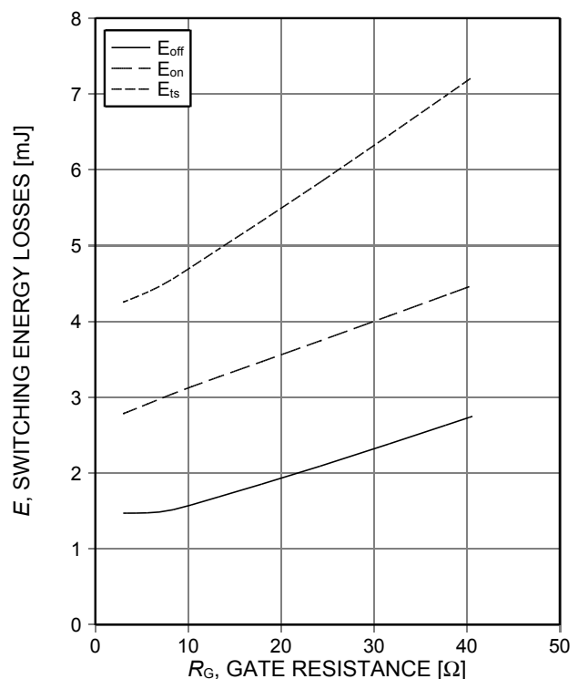
Figure 12. Typical switching energy losses as a function of gate resistance (inductive load, T_{vj}=150^\circ C , V_{CE}=400V , V_{GE}=0/15V , I_C=75A , dynamic test circuit in Figure E)
