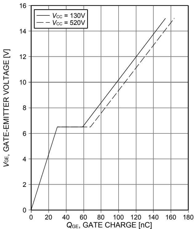
Figure 15. Typical gate charge ( I_C=75A )
