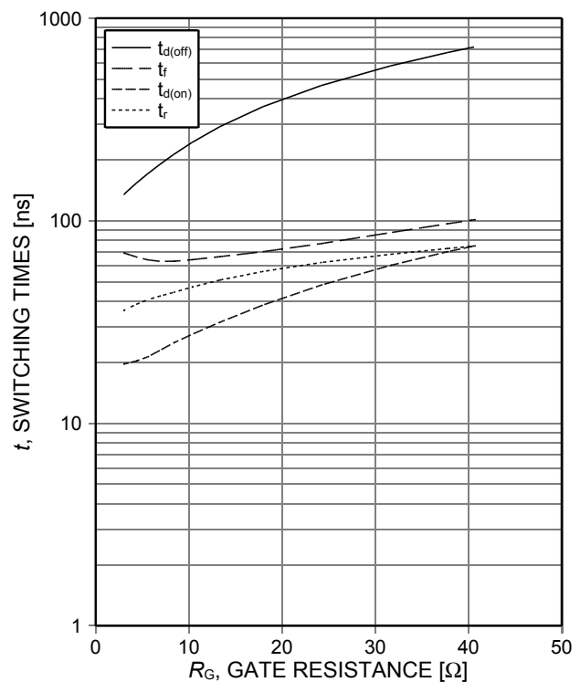
Figure 8. Typical switching times as a function of gate resistance (inductive load, T_{vj}=150^{\circ}C , V_{CE}=400V , V_{GE}=0/15V , I_C=75A , dynamic test circuit in Figure E)
