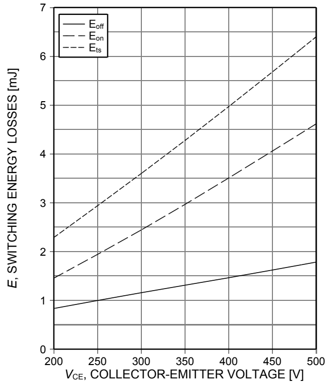
Figure 14. Typical switching energy losses as a function of collector emitter voltage (inductive load, T_{vj}=150^\circ C , V_{GE}=0/15V , I_C=75A , R_{Gon}=18\Omega , R_{Goff}=5.6\Omega , dynamic test circuit in Figure E)
