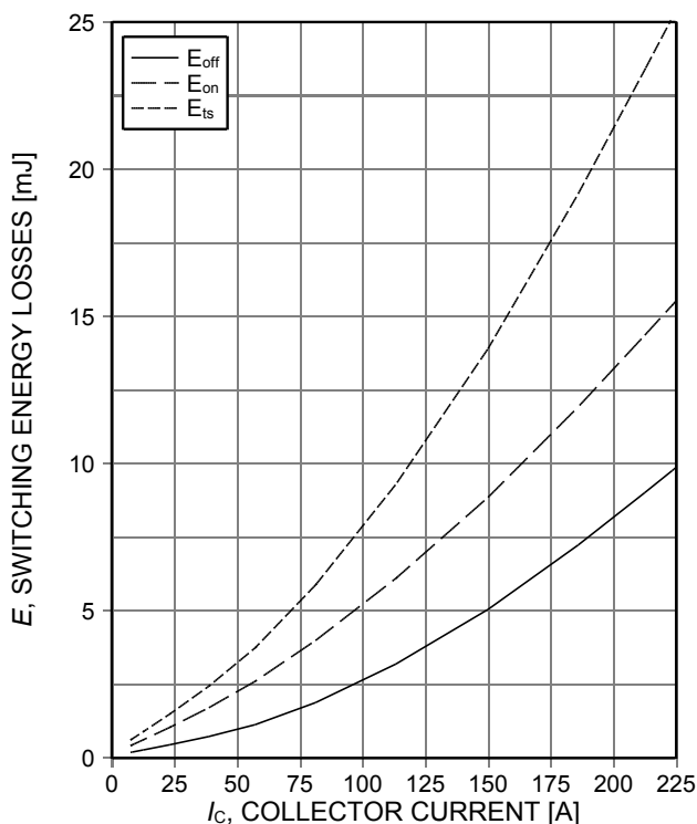
Figure 11. Typical switching energy losses as a function of collector current (inductive load, T_{vj}=150^\circ C , V_{CE}=400V , V_{GE}=0/15V , R_{Gon}=18\Omega , R_{Goff}=5.6\Omega , dynamic test circuit in Figure E)
