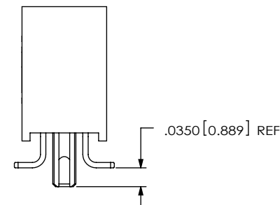
FIG 7 POLYAMIDE FILM PAD (4 POS MIN) SQW-110-01-XXX-D-VS-K SHOWN (DIFFERENT AS SHOWN, OTHERWISE SAME AS FIG 1)
