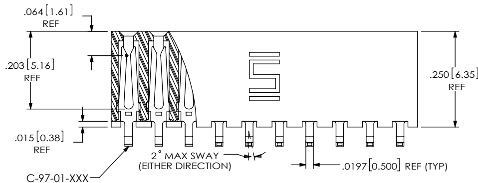
FIG 1 SQW-110-01-XXX-D-VS SHOWN
