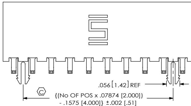
FIG 5 -A: MOLDED ALIGNMENT PIN (5 POS MIN) SQW-110-01-XXX-D-VS-A SHOWN (DIFFERENT AS SHOWN, OTHERWISE SAME AS FIG 1)
