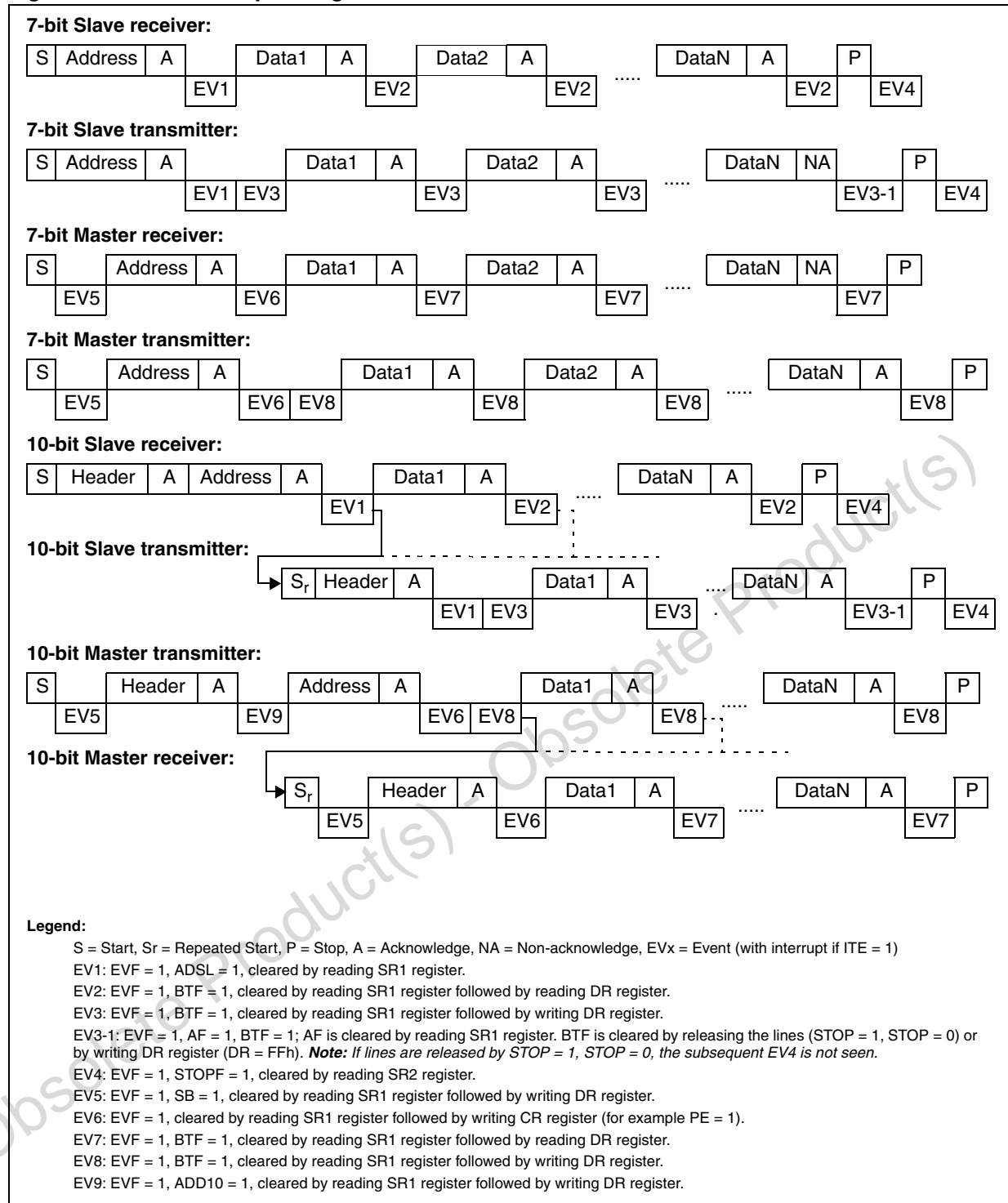
Figure 68. Transfer sequencing
