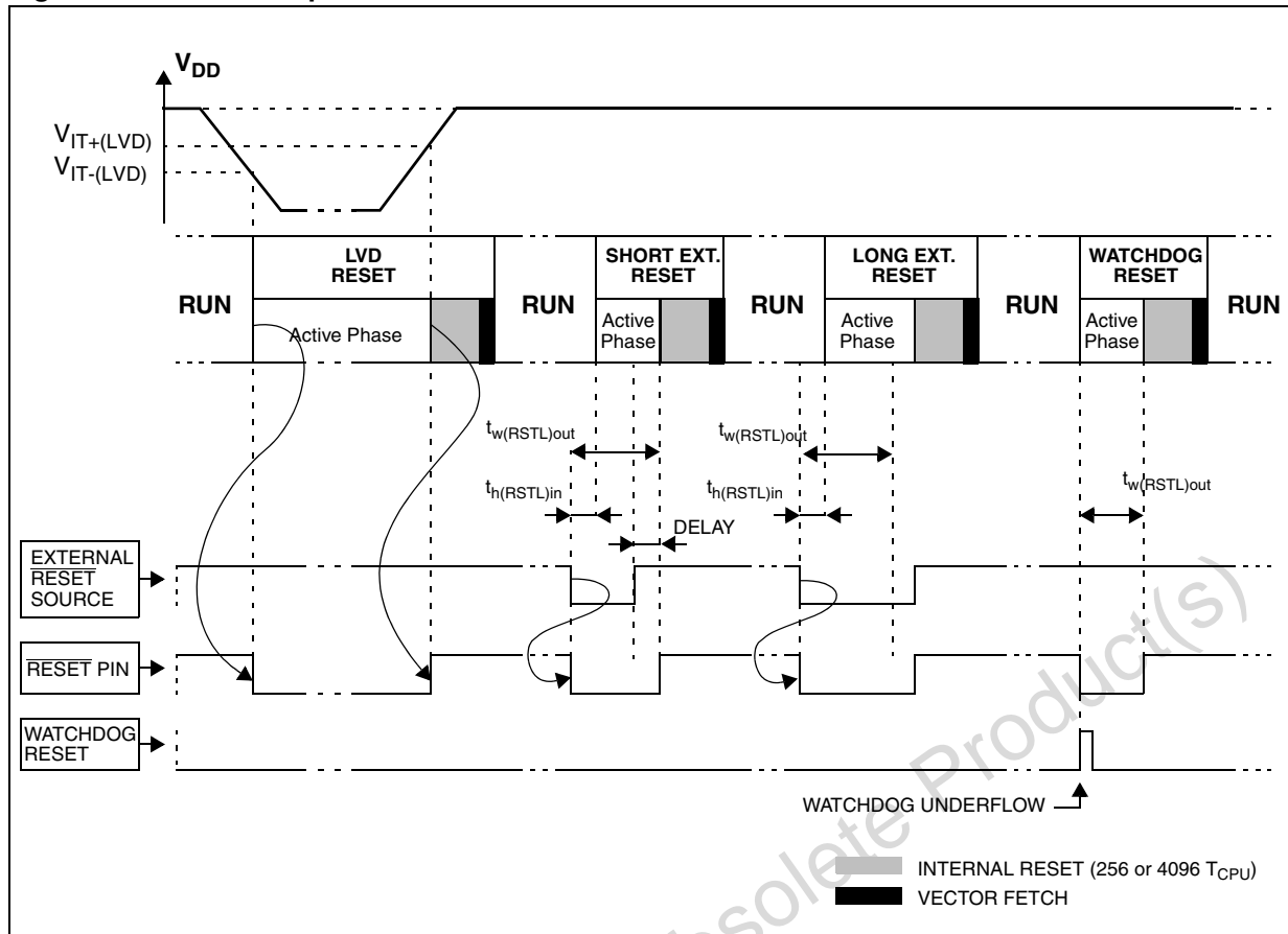
Figure 13. RESET sequences
