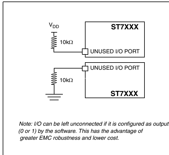
Figure 79. Unused I/O pins configured as input
