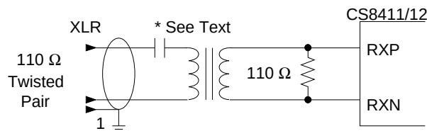
Figure 21. Professional Input Circuit
