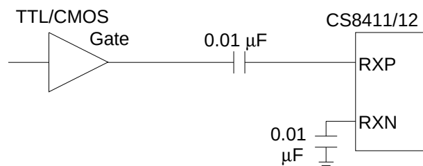
Figure 24. TTL/CMOS Interface
