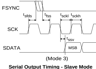
Serial Output Timing - Slave Mode
