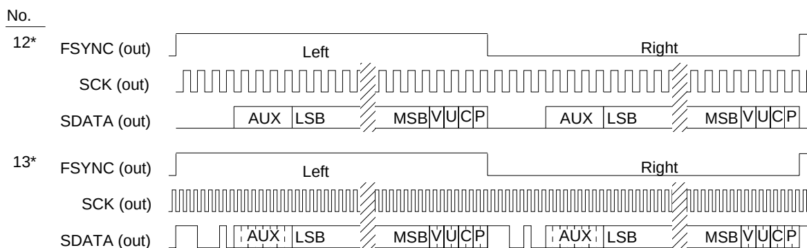
Figure 18. Special Audio Port Formats 12 and 13
