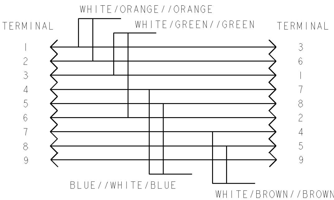
1 WIRING DIAGRAM Crossover
