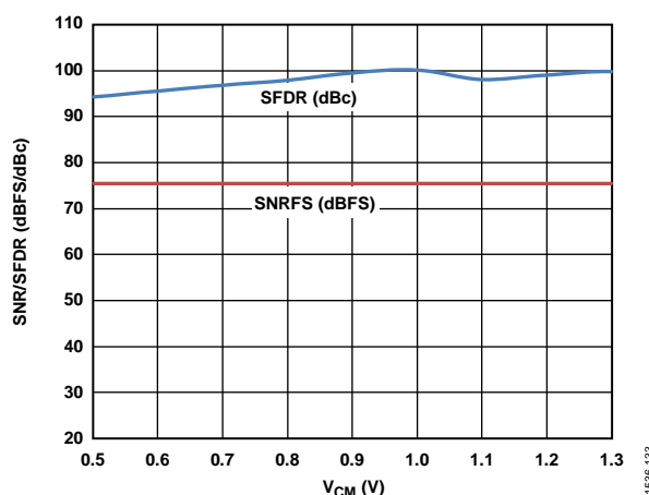
Figure 33. SNR/SFDR vs. Common-Mode Voltage, f_{IN} = 9.7 \text{ MHz} , f_{SAMPLE} = 65 \text{ MSPS}
