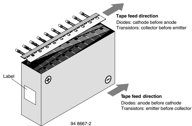
Fig. 31 - Tape Direction
