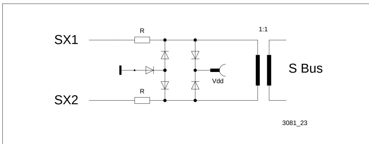
Figure 24 External Circuitry for Transmitter
