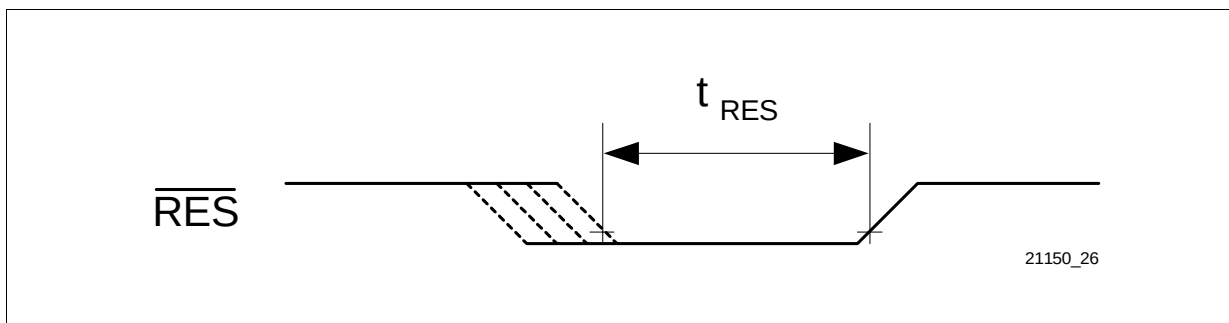
Figure 73 Reset Signal \overline{\text{RES}}
