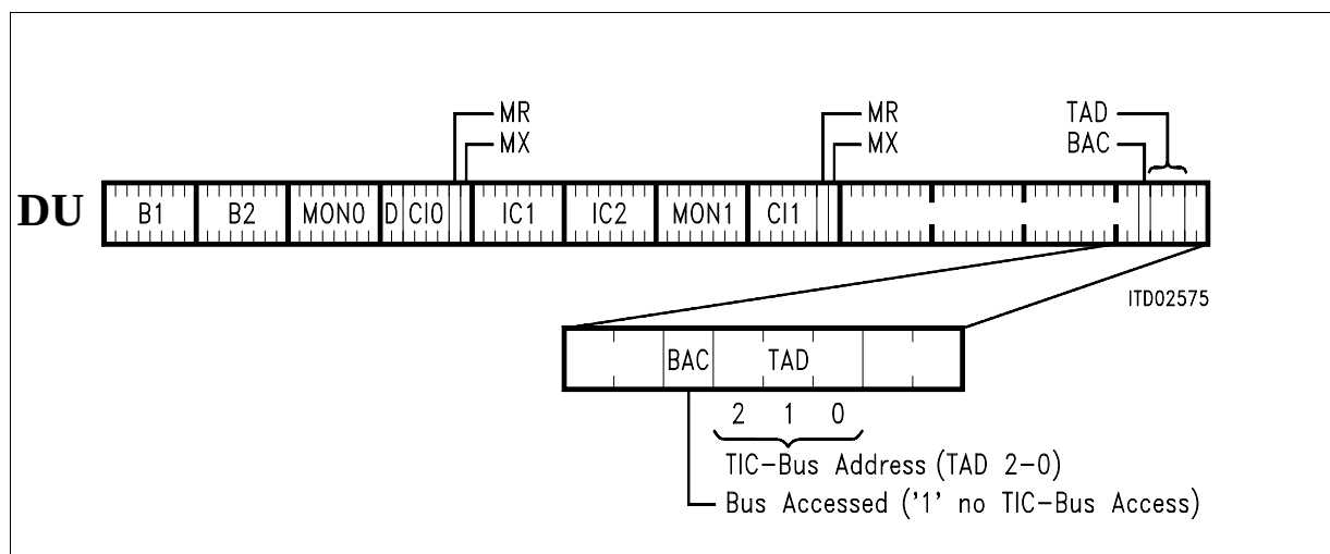
Figure 60 Structure of Last Octet of Ch2 on DU
