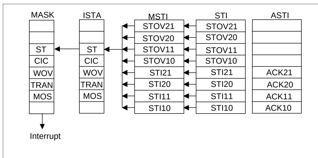
Figure 48 Interrupt Structure of the Synchronous Data Transfer
