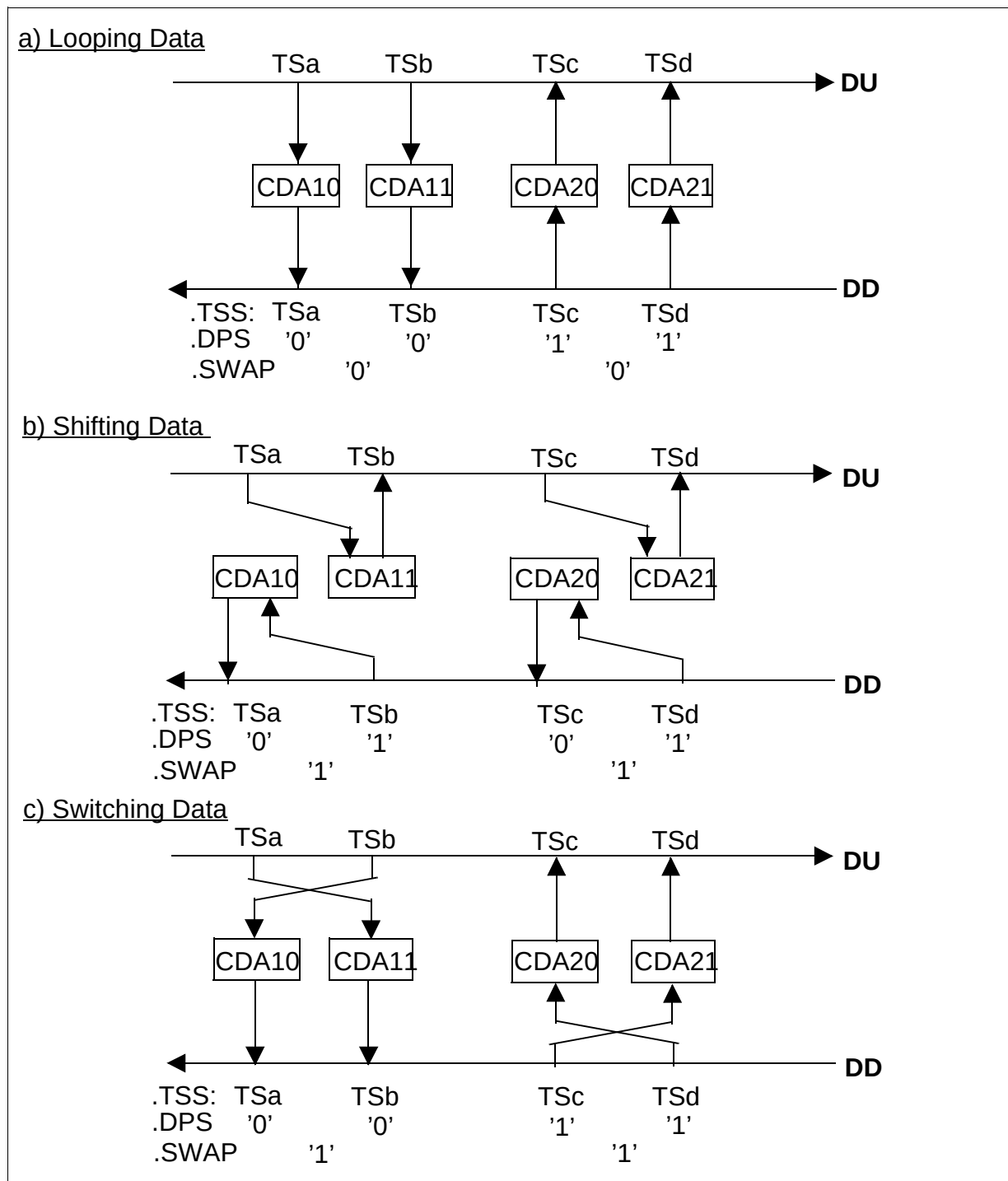
Figure 44 Examples for Data Access via CDAxy Registers
