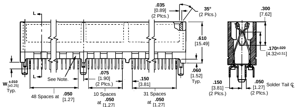
Section L-L
